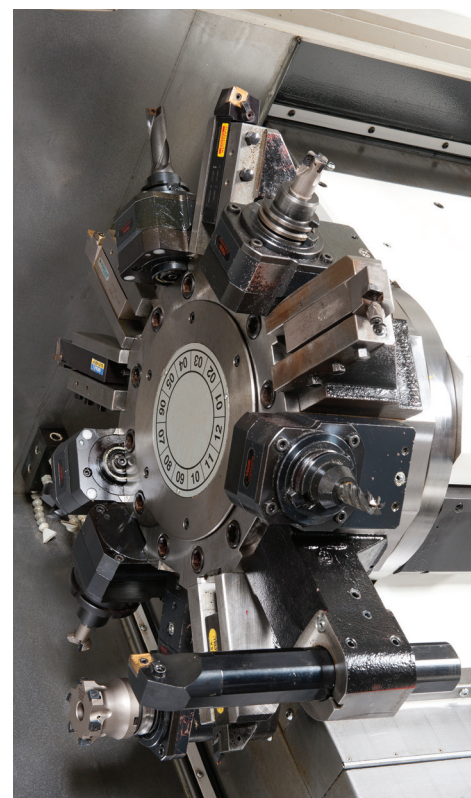
Multi-Tasking Turret
