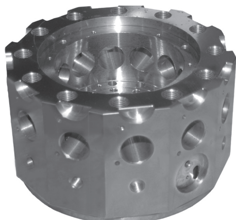
Machined VDI Turret
