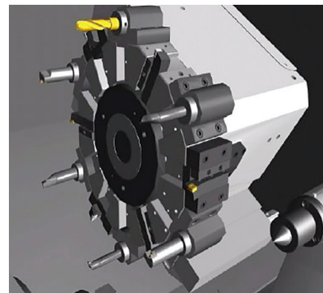
Standard Turret
